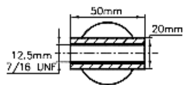
Magnification of A
